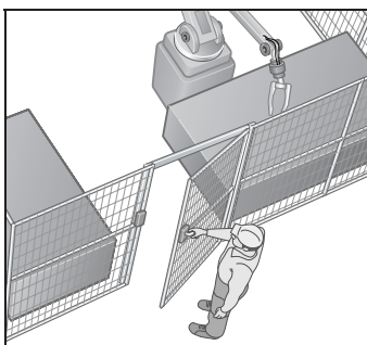
The Category II SAFE LOCK, provides excellent levels of safety. Only in state 3 is an electrical signal transmitted to allow the machinery to start.
